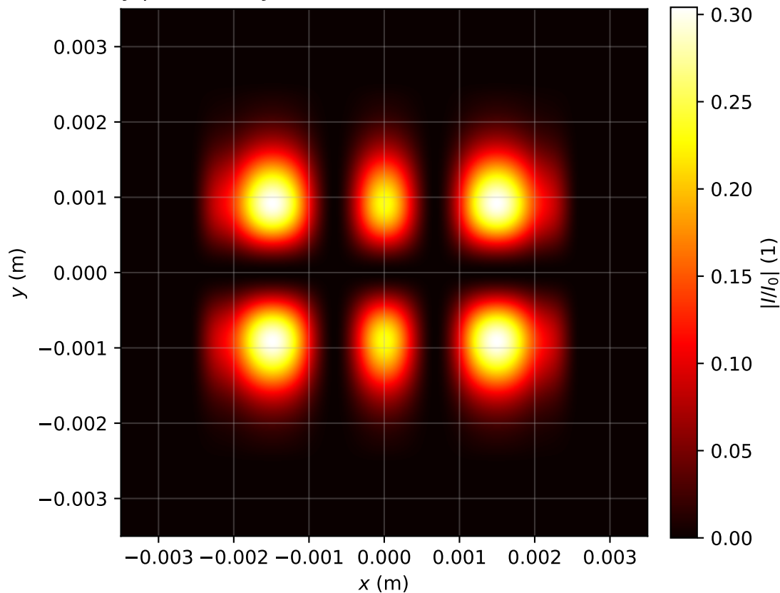
Intensity profile I(x, y, z = 3.184)/I_0 , P_{in}=0.5P_{cr} , artificial time
